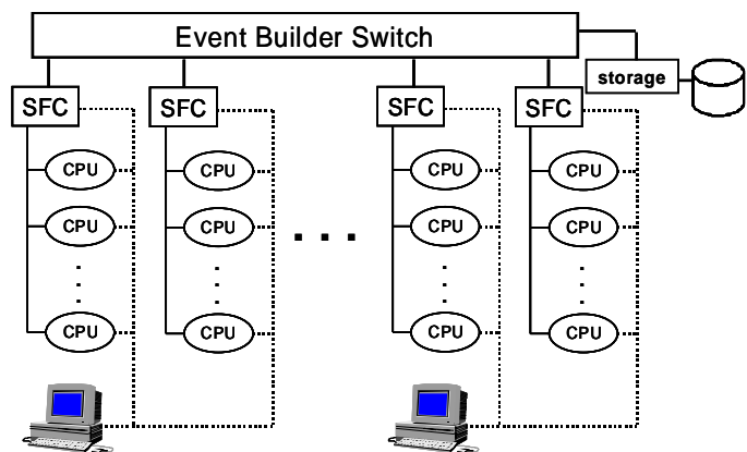
Fig. 8. Schematic view of the control of the Event Filter Farm
