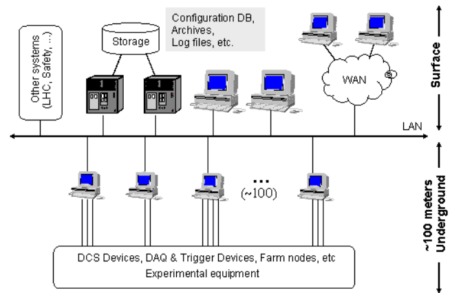
Fig. 4. LHCb's ECS Hardware Architecture
