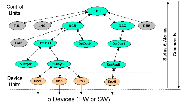
Fig. 3. LHCb's ECS Software Architecture
