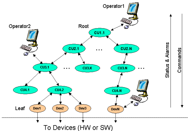
Fig. 2. JCOP Software Architecture
