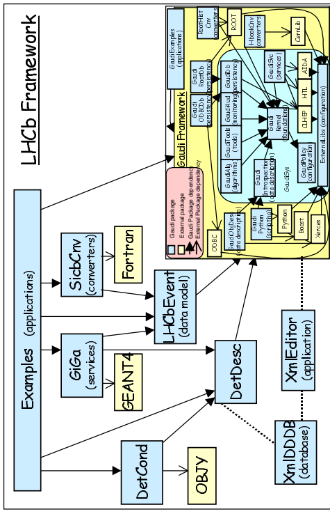
Figure 16.2 Package structure of the LHCb Gaudi software
